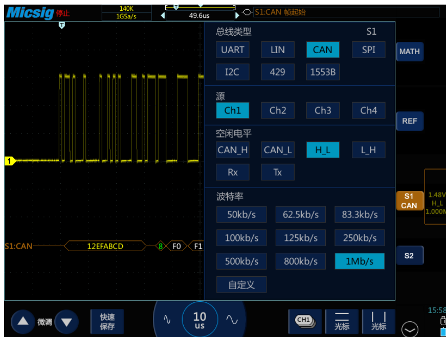
图13-9 CAN 总线配置菜单
